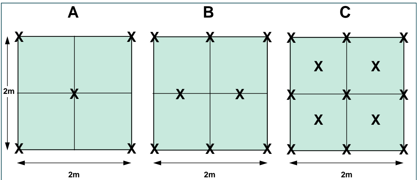
Figure 2 - Fixing pattern
